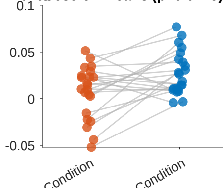
Session Means (p=0.0125)
